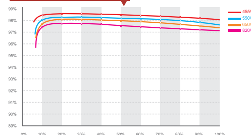
Growatt CP500TL efficiency
